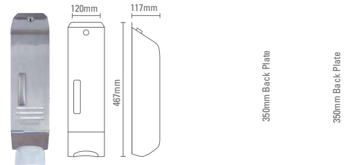
STAINLESS STEEL DISPENSER - 4405 Lockable, where a polished steel finish is required
