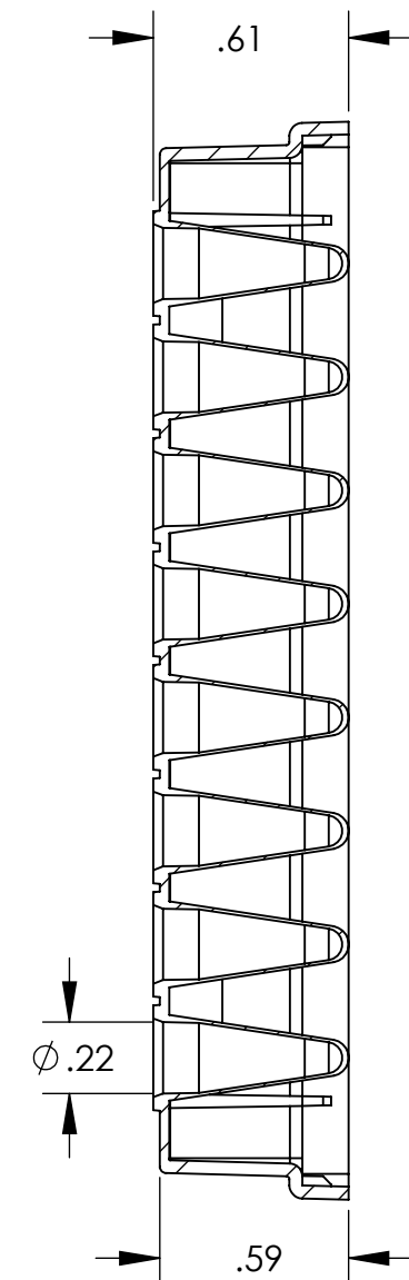
SECTION F-F
